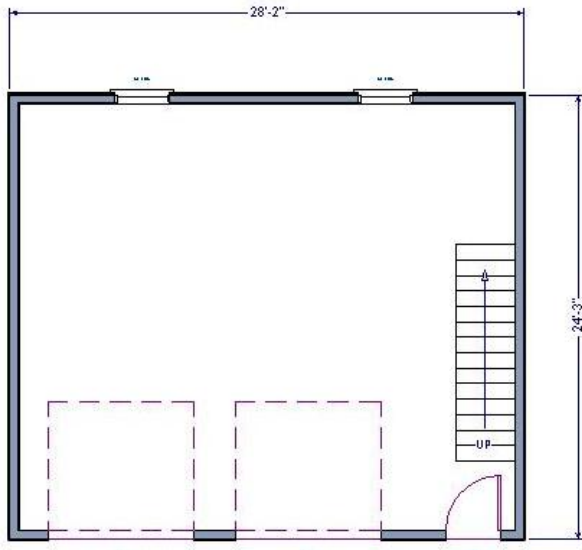
2 Car Garage 683 sq ft
